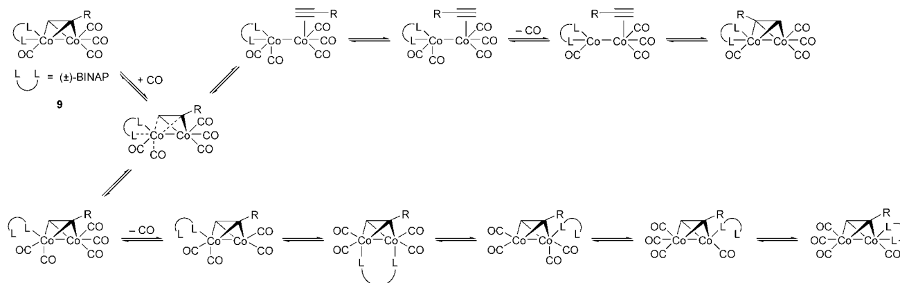
Scheme 12. Two possible isomerization pathways for complexes of type 9 .
