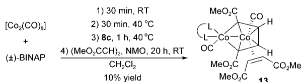
Scheme 14. Synthesis of cobaltacyclopentadiene 13 .
