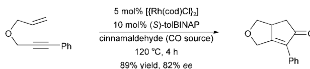
Scheme 6. The enantioselective, rhodium-catalyzed PKR with cinnamaldehyde as the CO source. [12]
