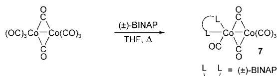
Scheme 8. Synthesis of [\text{Co}_2(\text{binap})(\text{CO})_6] .
