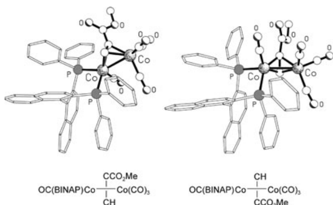
Figure 2. The molecular structures of 9c maj (left) and 9c min (right).
