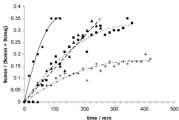
Figure 4. Inverse gated ^{31}\text{P} NMR isomerization experiments with 9c_{\text{maj}} (◆ —, \text{CO}/75^\circ\text{C} ; ▲ ---, \text{N}_2/75^\circ\text{C} ; ■ ----, \text{CO}/60^\circ\text{C} ; + -.-, \text{N}_2/60^\circ\text{C} ).
