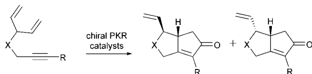
Scheme 7. Desymmetrization of meso -dienynes by asymmetric Pauson-Khand catalysis. [13]
