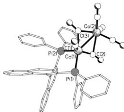
Figure 1. The molecular structure of 7 .
