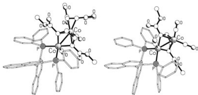
Figure 5. The molecular structures of 12 (left) and 13 (right).
