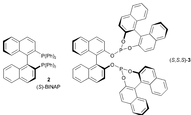
Scheme 3. Our report of improved conditions for the asymmetric, cobalt-catalyzed PKR. [8]
