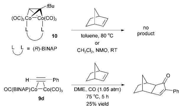
Scheme 11. Laschat's [17] report of the inactivity of [\text{Co}_2(3,3\text{-dimethylbutyne})(\text{CO})_6] in the stoichiometric PKR (top). Our example of 9d in the stoichiometric PKR (bottom).
