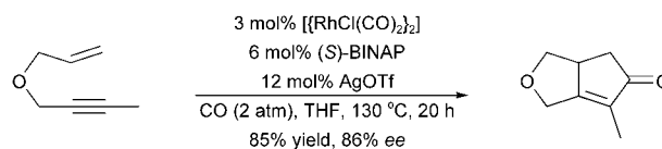
Scheme 4. The enantioselective, catalytic PKR with rhodium. [9]
