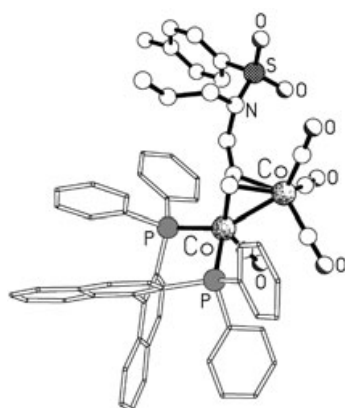
Figure 3. The molecular structure of 9e .
