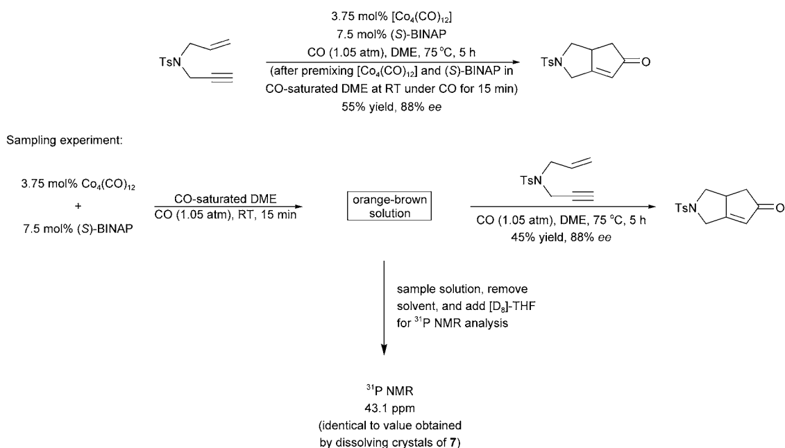
Scheme 9. A typical Pauson–Khand reaction (top) and the same reaction conducted with sampling of the precatalyst solution (bottom).
