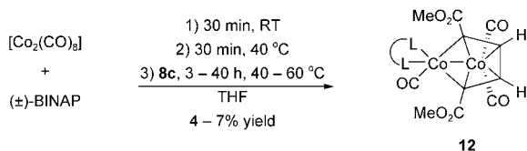
Scheme 13. Synthesis of cobaltacyclopentadiene 12 .
