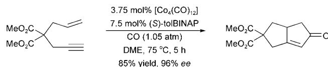
Scheme 3. Our report of improved conditions for the asymmetric, cobalt-catalyzed PKR. [8]
